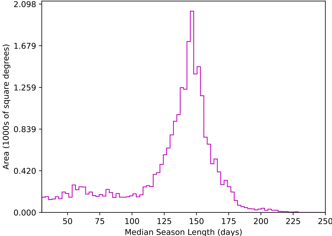
too_elab_heavy_r128_d2_gz_v3.4_10yrs All sky z band: Median Season Length
