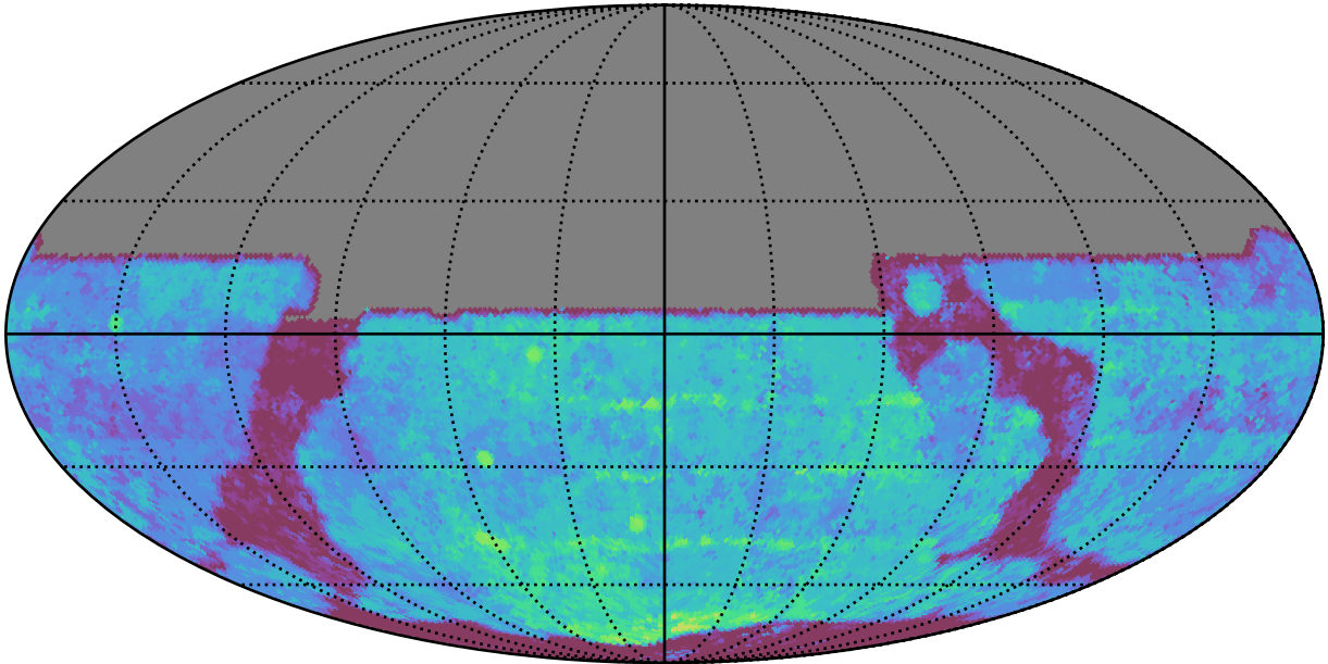
too_elab_heavy_r128_d2_gz_v3.4_10yrs All sky y band: Median Season Length
