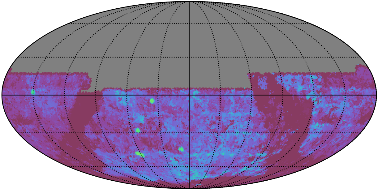
too_elab_heavy_r128_d2_gz_v3.4_10yrs All sky u band: Median Season Length
