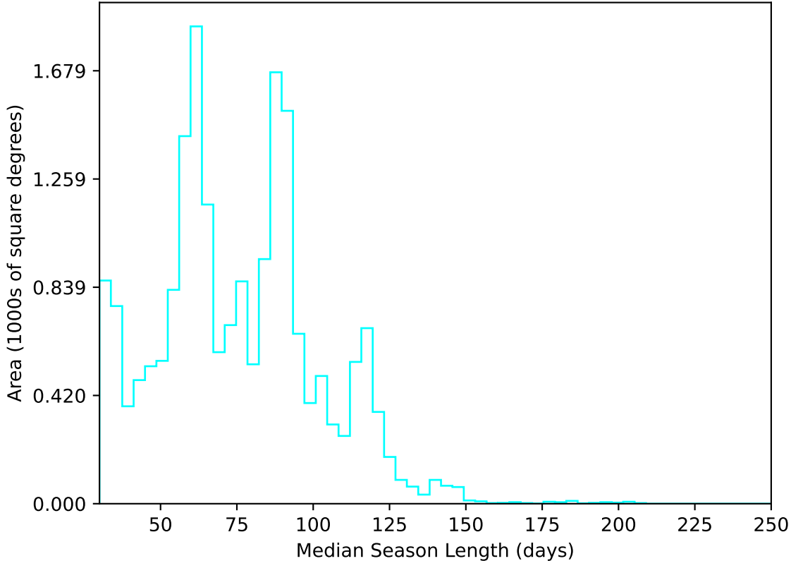
too_elab_heavy_r128_d2_gz_v3.4_10yrs All sky u band: Median Season Length
