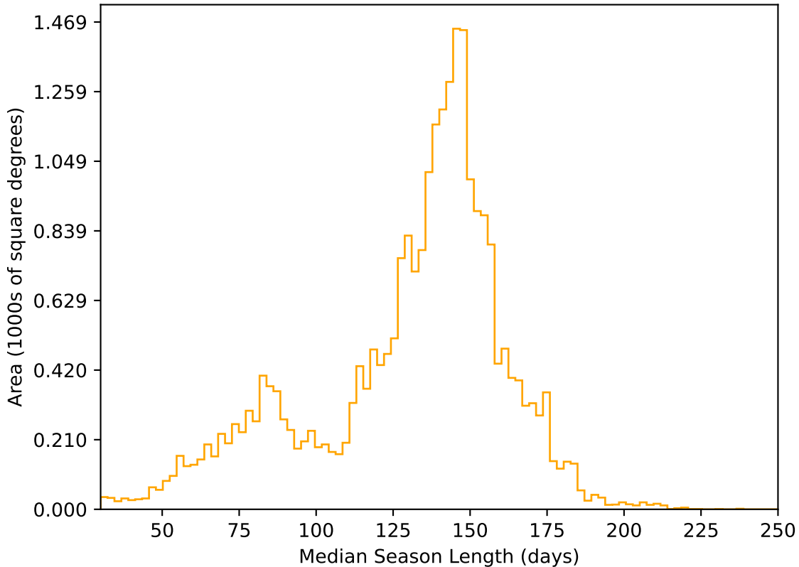
too_elab_heavy_r128_d2_gz_v3.4_10yrs All sky r band: Median Season Length
