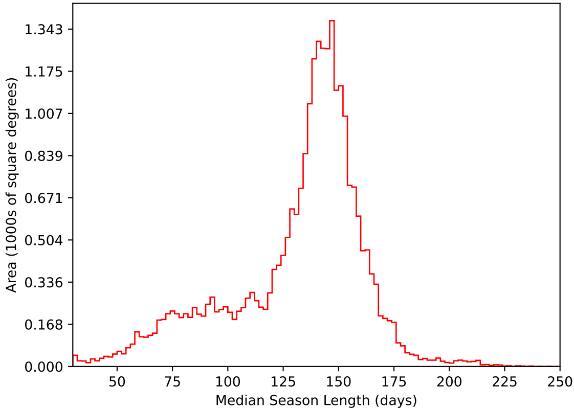
too_elab_heavy_r128_d2_gz_v3.4_10yrs All sky i band: Median Season Length
