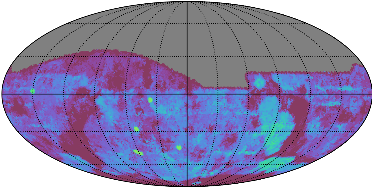
too_elab_heavy_r128_d2_gz_v3.4_10yrs All sky g band: Median Season Length
