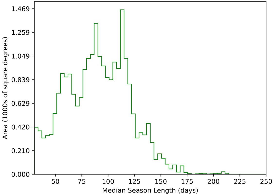
too_elab_heavy_r128_d2_gz_v3.4_10yrs All sky g band: Median Season Length
