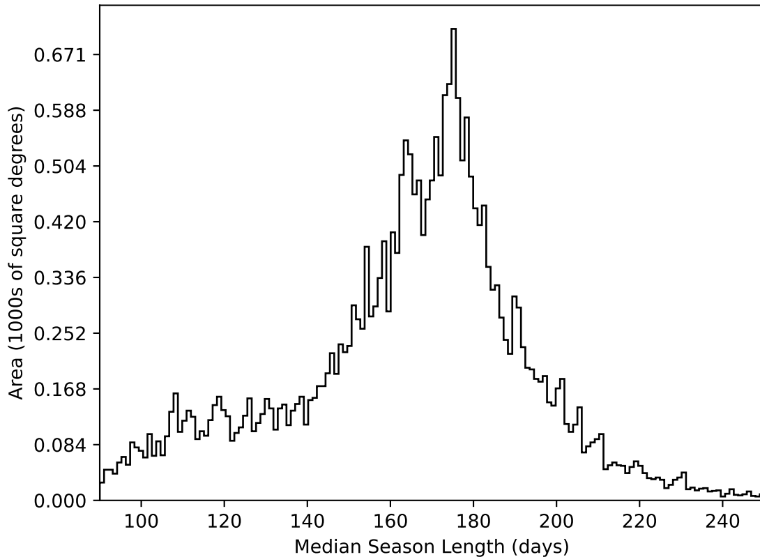
too_elab_heavy_r128_d2_gz_v3.4_10yrs All sky all bands: Median Season Length
