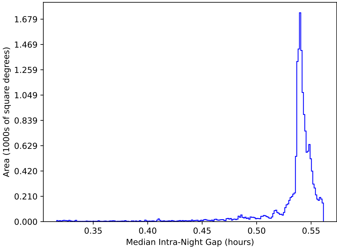
too_elab_heavy_r128_d2_gz_v3.4_10yrs WFD: Median Intra-Night Gap
