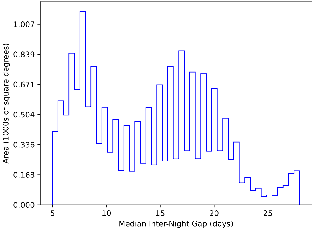
too_elab_heavy_r128_d2_gz_v3.4_10yrs WFD y band: Median Inter-Night Gap
