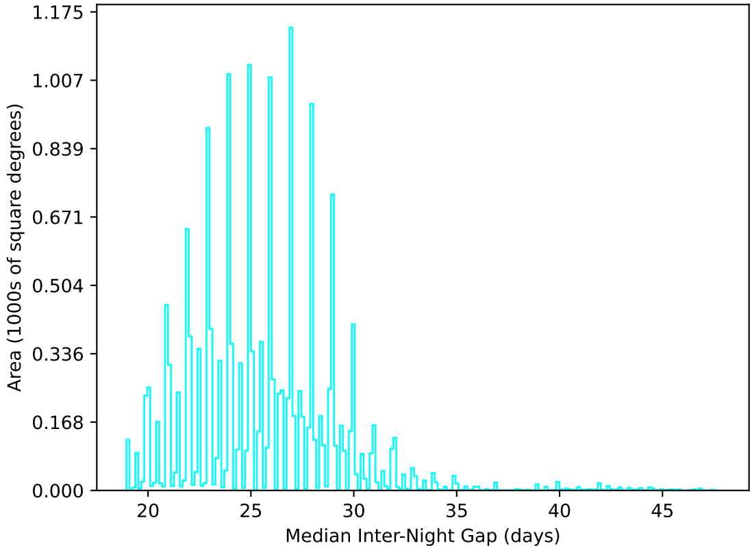
too_elab_heavy_r128_d2_gz_v3.4_10yrs WFD u band: Median Inter-Night Gap
