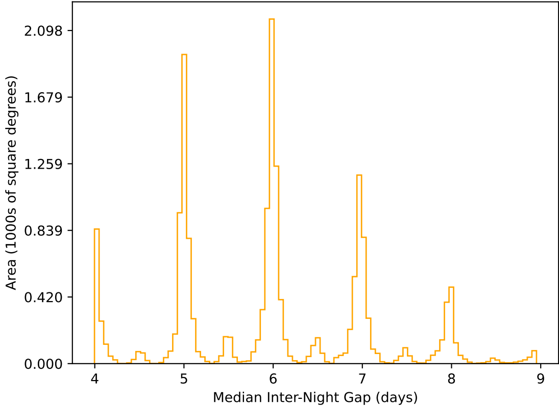
too_elab_heavy_r128_d2_gz_v3.4_10yrs WFD r band: Median Inter-Night Gap
