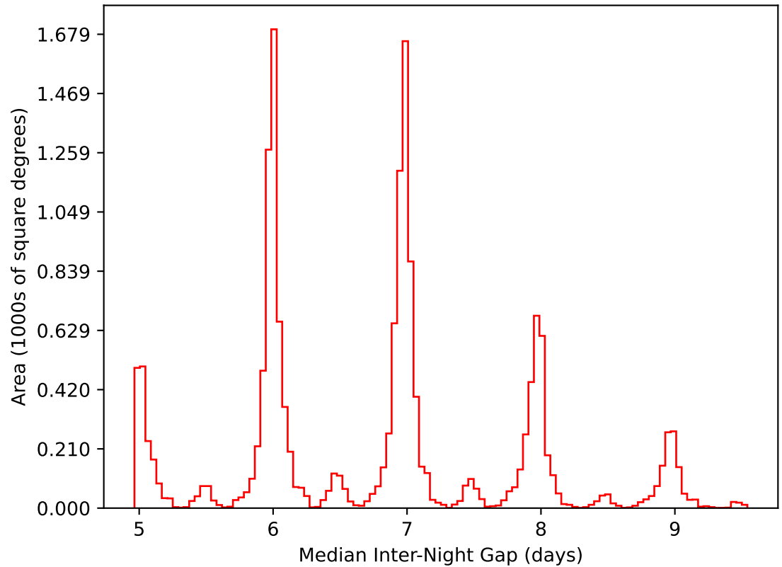
too_elab_heavy_r128_d2_gz_v3.4_10yrs WFD i band: Median Inter-Night Gap
