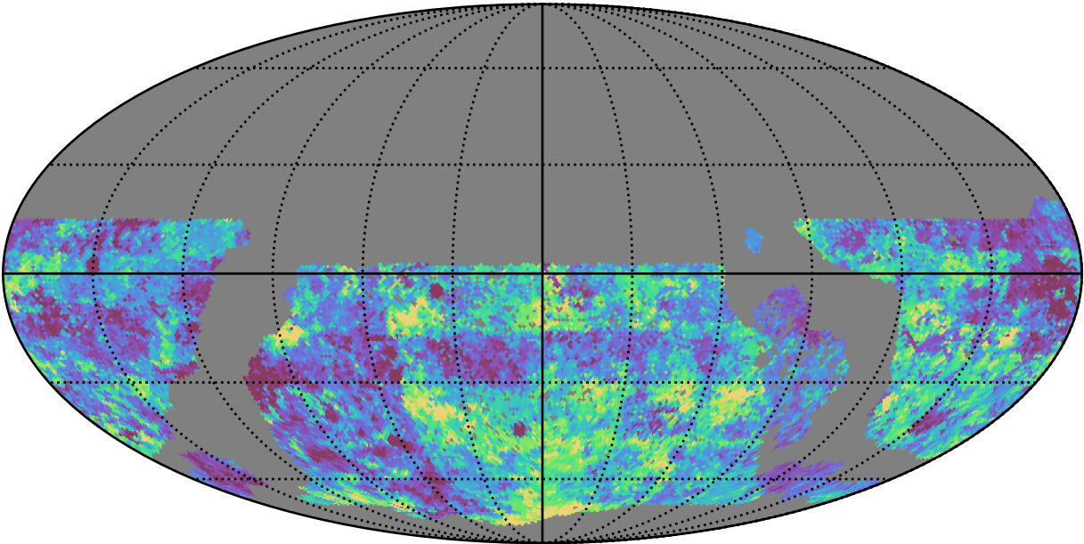
too_elab_heavy_r128_d2_gz_v3.4_10yrs WFD g band: Median Inter-Night Gap
