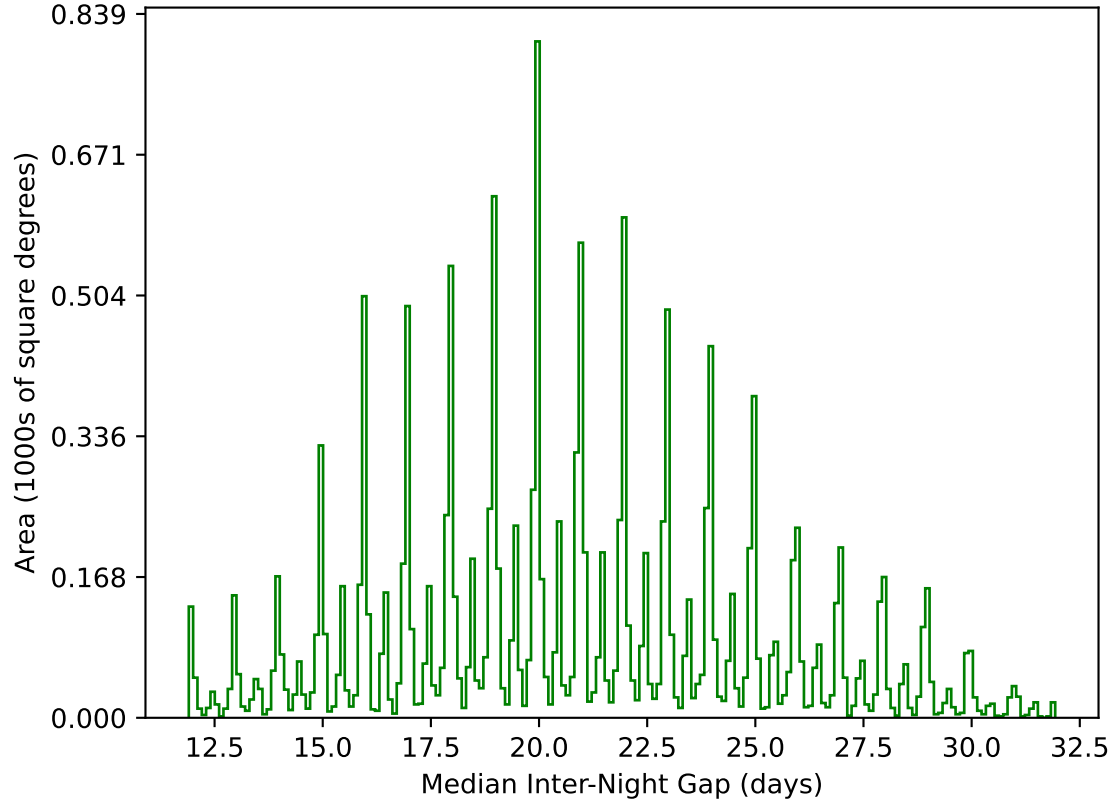
too_elab_heavy_r128_d2_gz_v3.4_10yrs WFD g band: Median Inter-Night Gap
