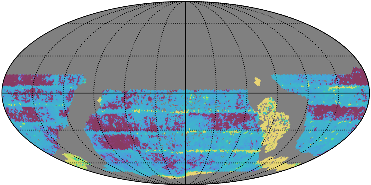
too_elab_heavy_r128_d2_gz_v3.4_10yrs WFD all bands: Median Inter-Night Gap
