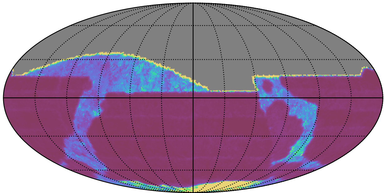
too_elab_heavy_r128_d2_gz_v3.4_10yrs All sky i band: Median Inter-Night Gap
