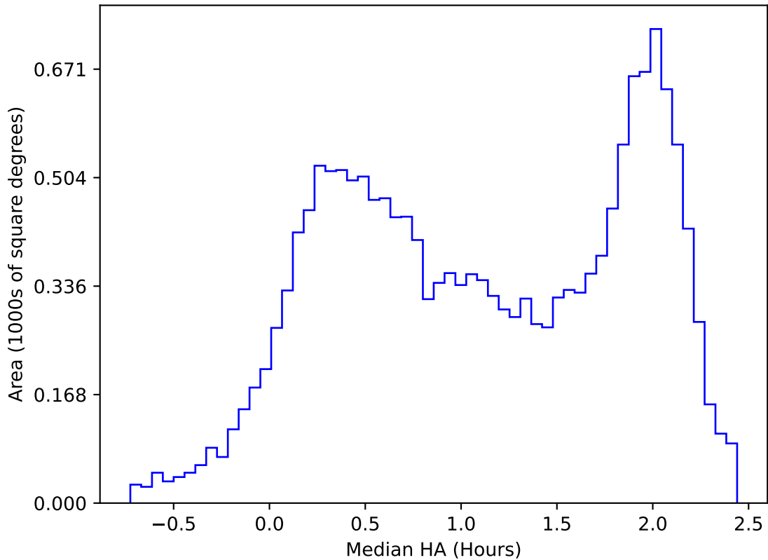
too_elab_heavy_r128_d2_gz_v3.4_10yrs WFD z band: Median HA
