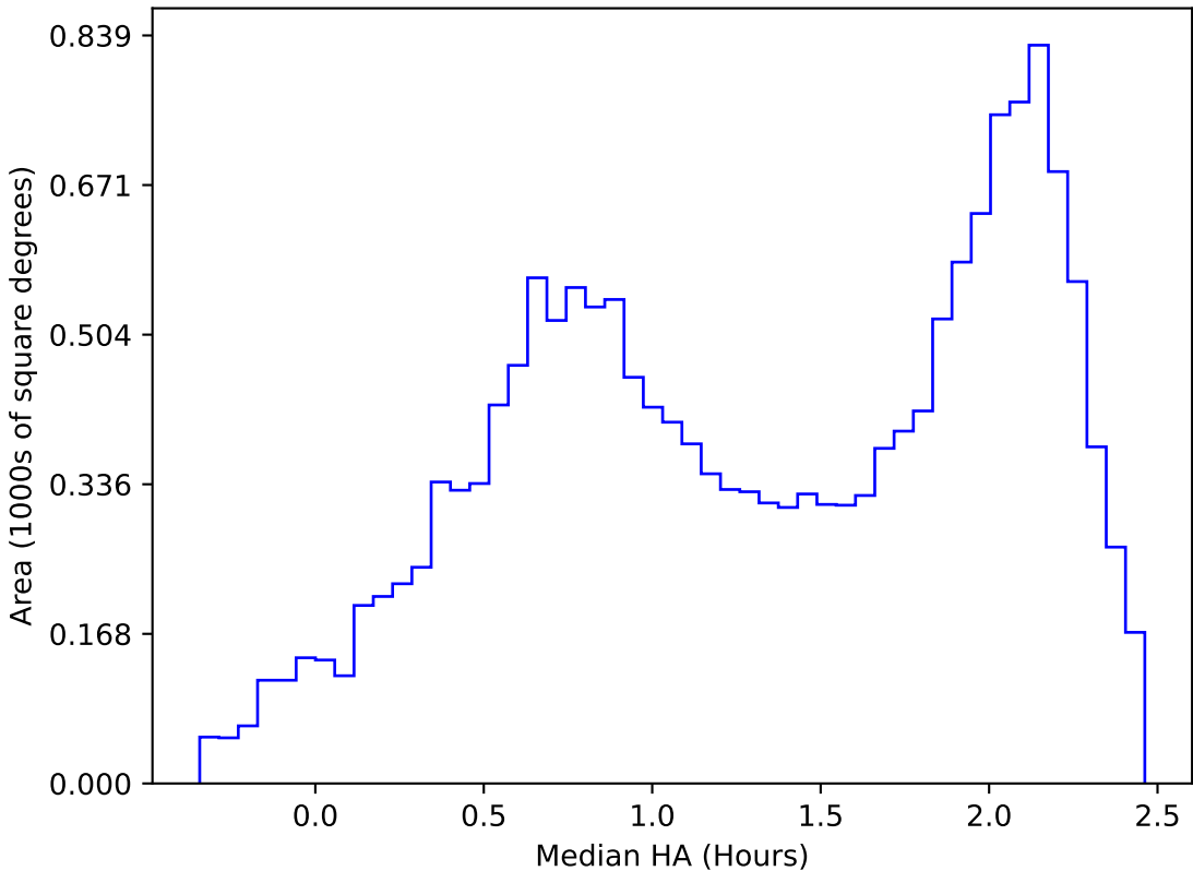
too_elab_heavy_r128_d2_gz_v3.4_10yrs WFD y band: Median HA
