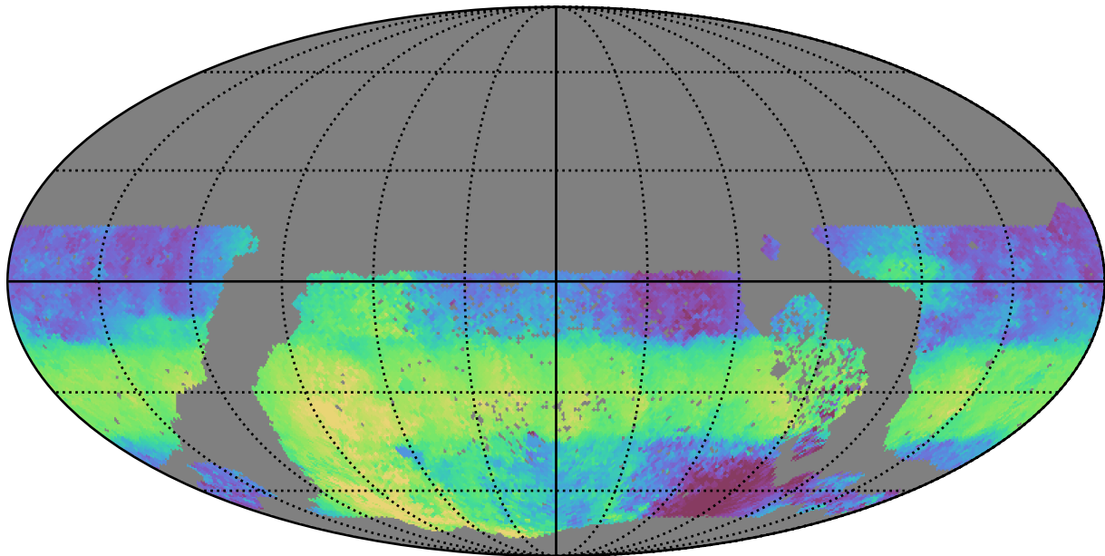
too_elab_heavy_r128_d2_gz_v3.4_10yrs WFD u band: Median HA
