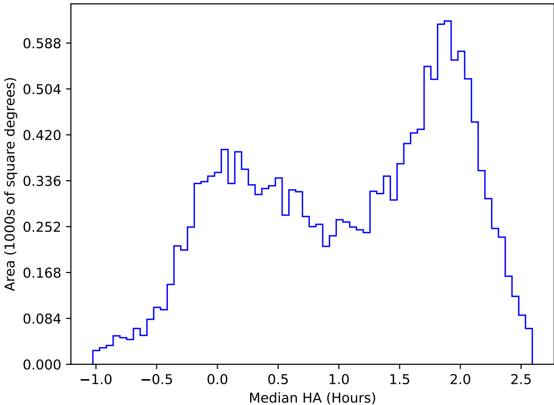
too_elab_heavy_r128_d2_gz_v3.4_10yrs WFD u band: Median HA
