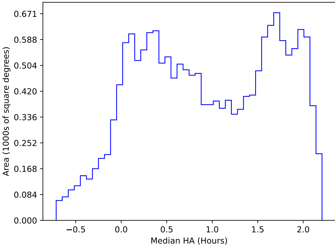
too_elab_heavy_r128_d2_gz_v3.4_10yrs WFD r band: Median HA
