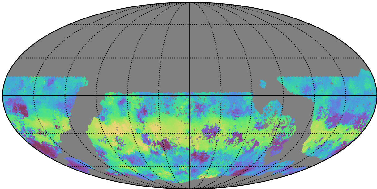
too_elab_heavy_r128_d2_gz_v3.4_10yrs WFD g band: Median HA
