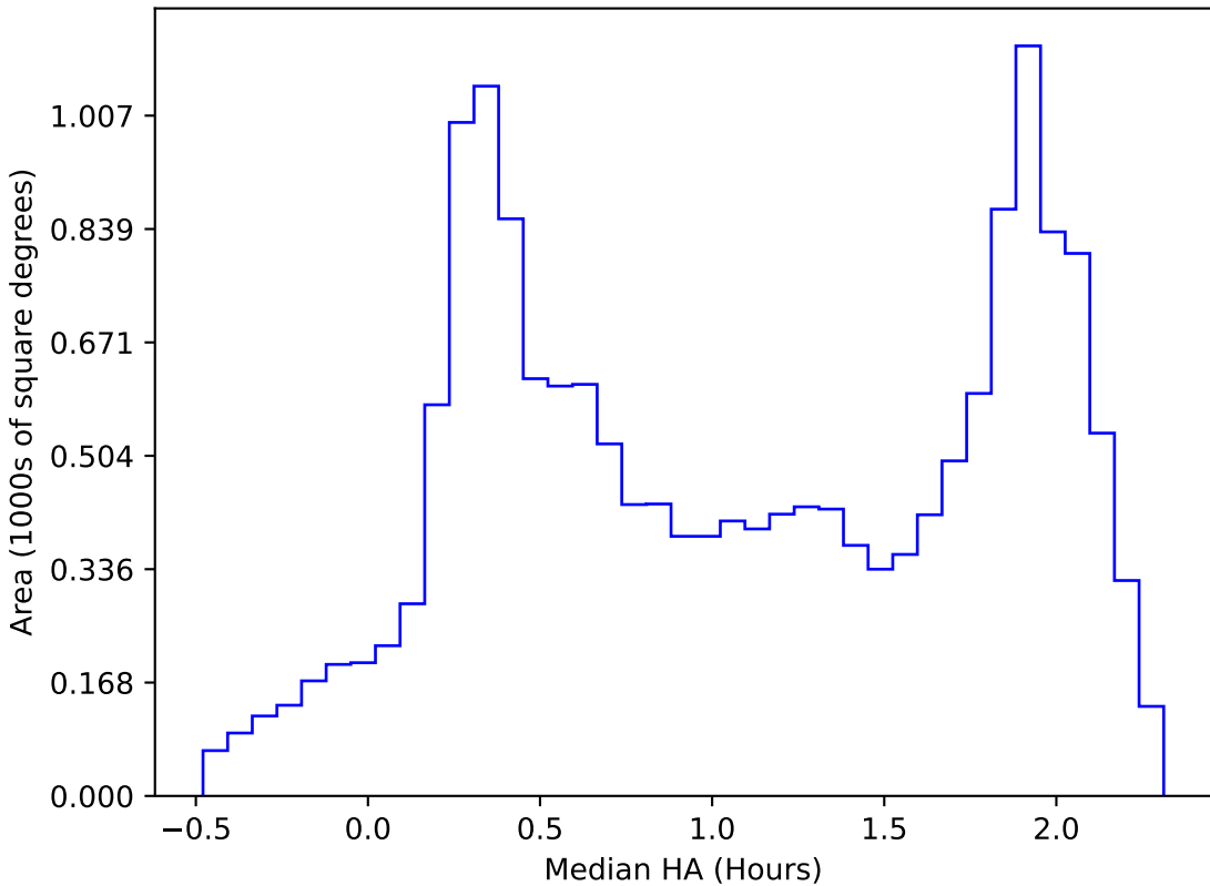
too_elab_heavy_r128_d2_gz_v3.4_10yrs WFD all bands: Median HA
