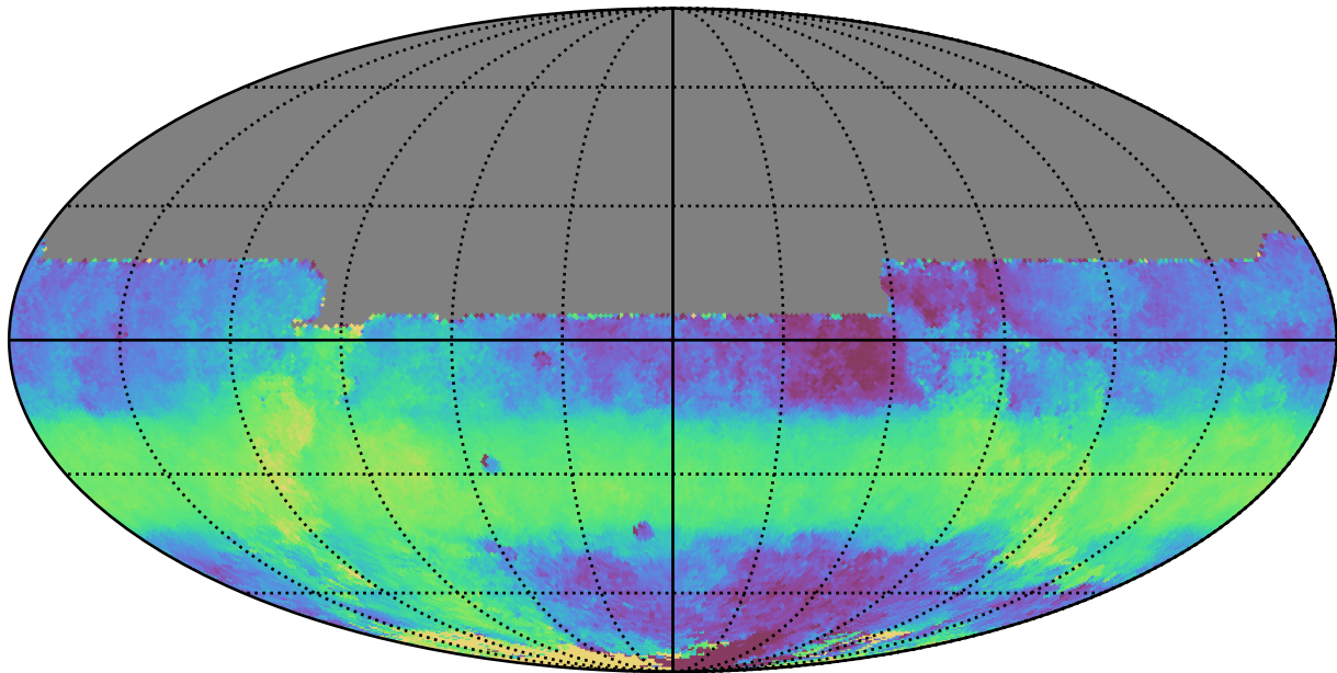
too_elab_heavy_r128_d2_gz_v3.4_10yrs All sky y band: Median HA
