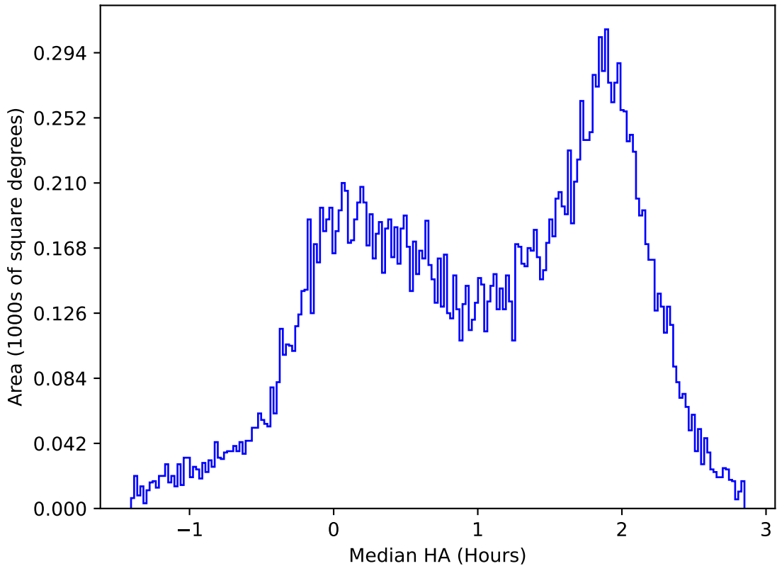
too_elab_heavy_r128_d2_gz_v3.4_10yrs All sky u band: Median HA
