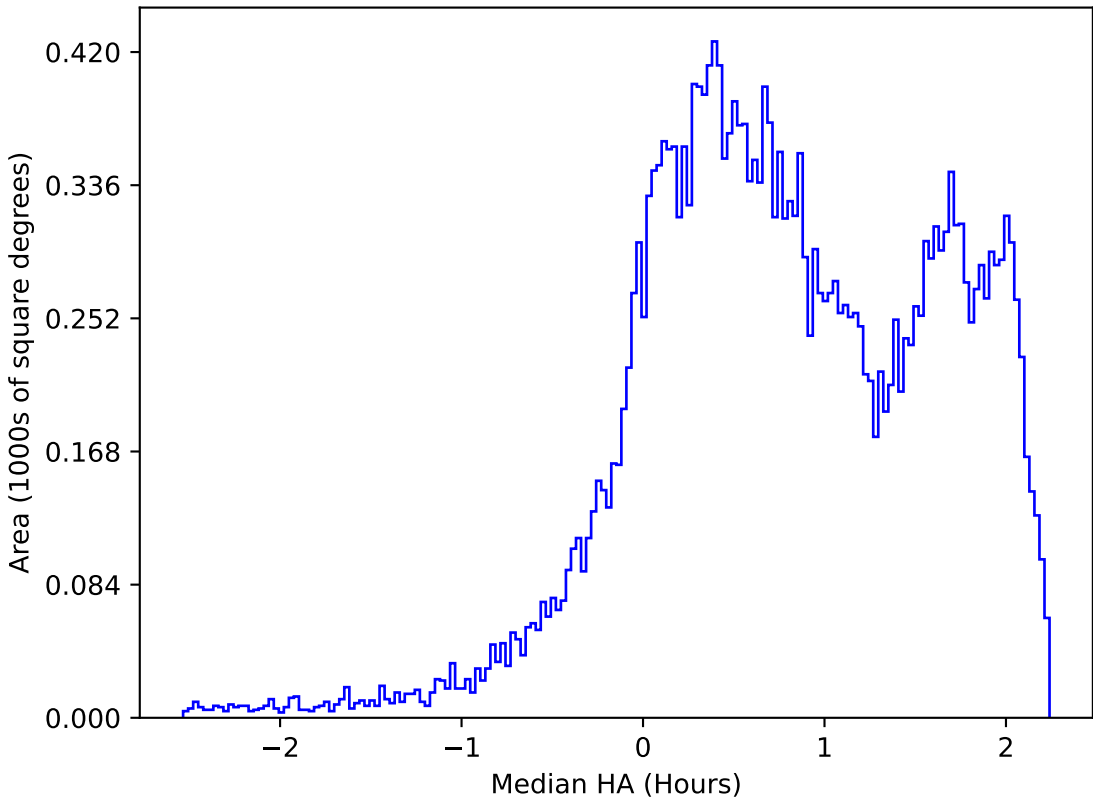
too_elab_heavy_r128_d2_gz_v3.4_10yrs All sky r band: Median HA
