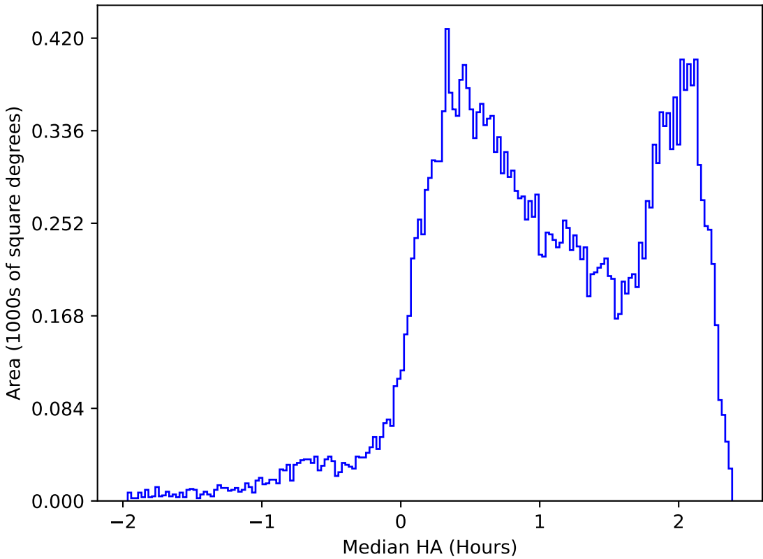
too_elab_heavy_r128_d2_gz_v3.4_10yrs All sky i band: Median HA
