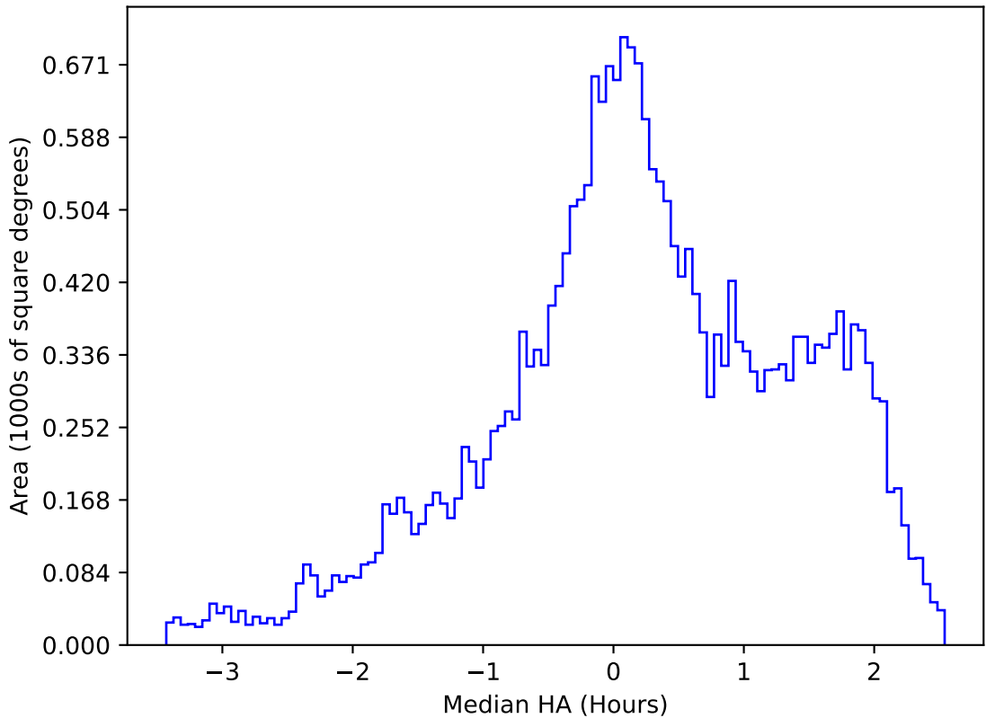
too_elab_heavy_r128_d2_gz_v3.4_10yrs All sky g band: Median HA
