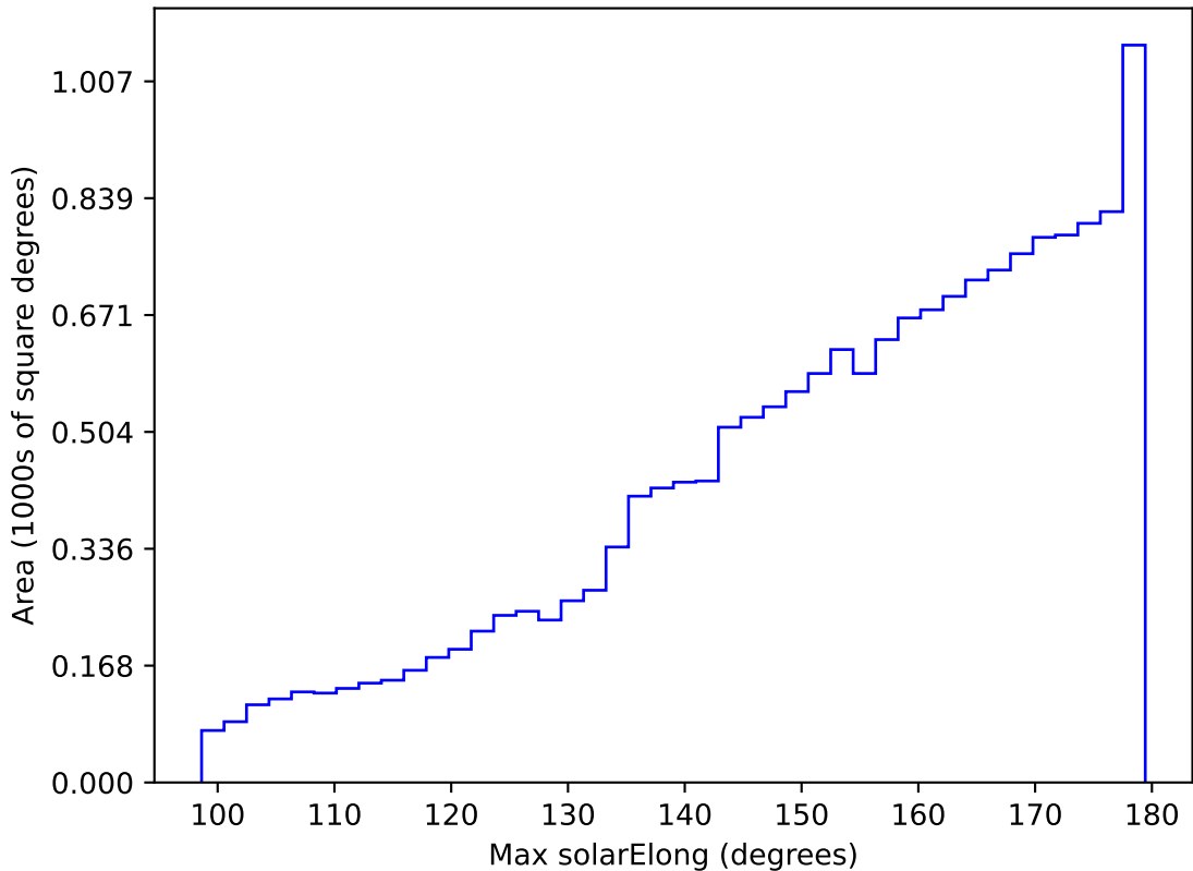
too_elab_heavy_r128_d2_gz_v3.4_10yrs WFD r band: Max solarElong
