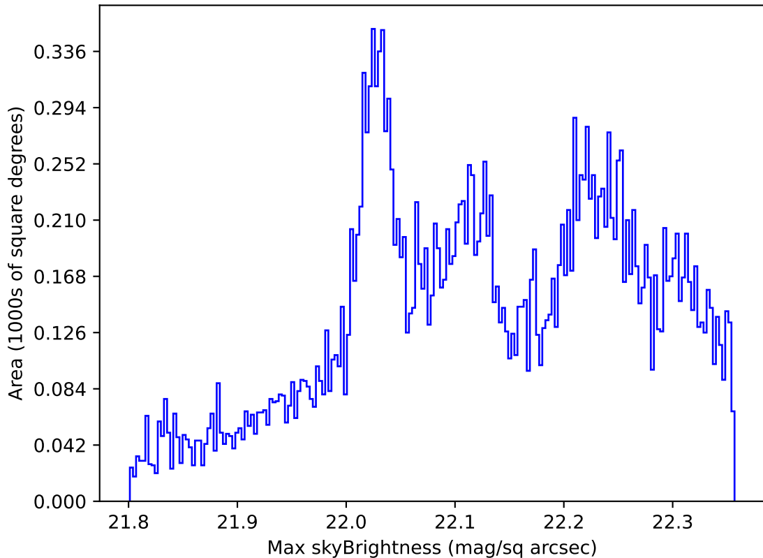
too_elab_heavy_r128_d2_gz_v3.4_10yrs All sky g band: Max skyBrightness
