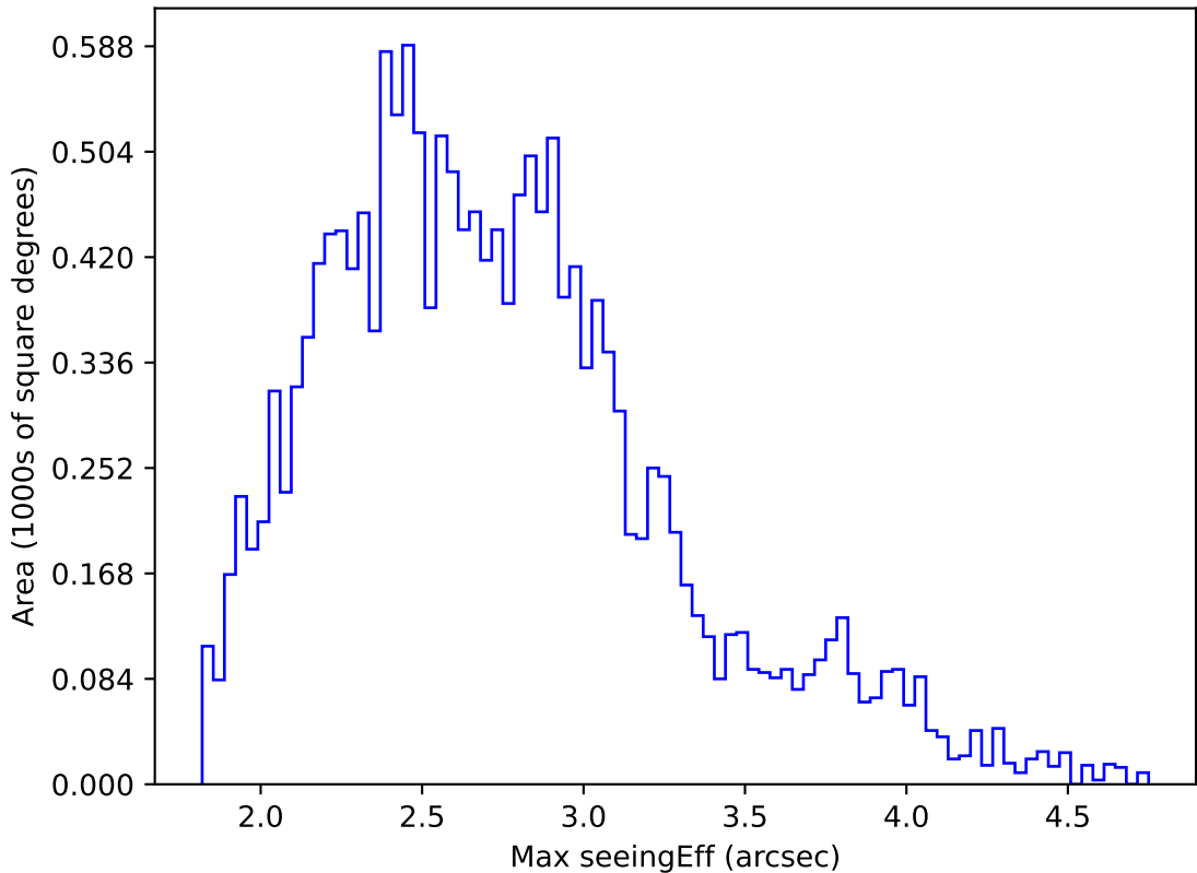
too_elab_heavy_r128_d2_gz_v3.4_10yrs WFD r band: Max seeingEff
