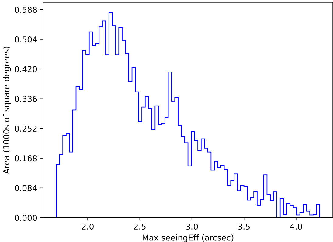
too_elab_heavy_r128_d2_gz_v3.4_10yrs WFD g band: Max seeingEff
