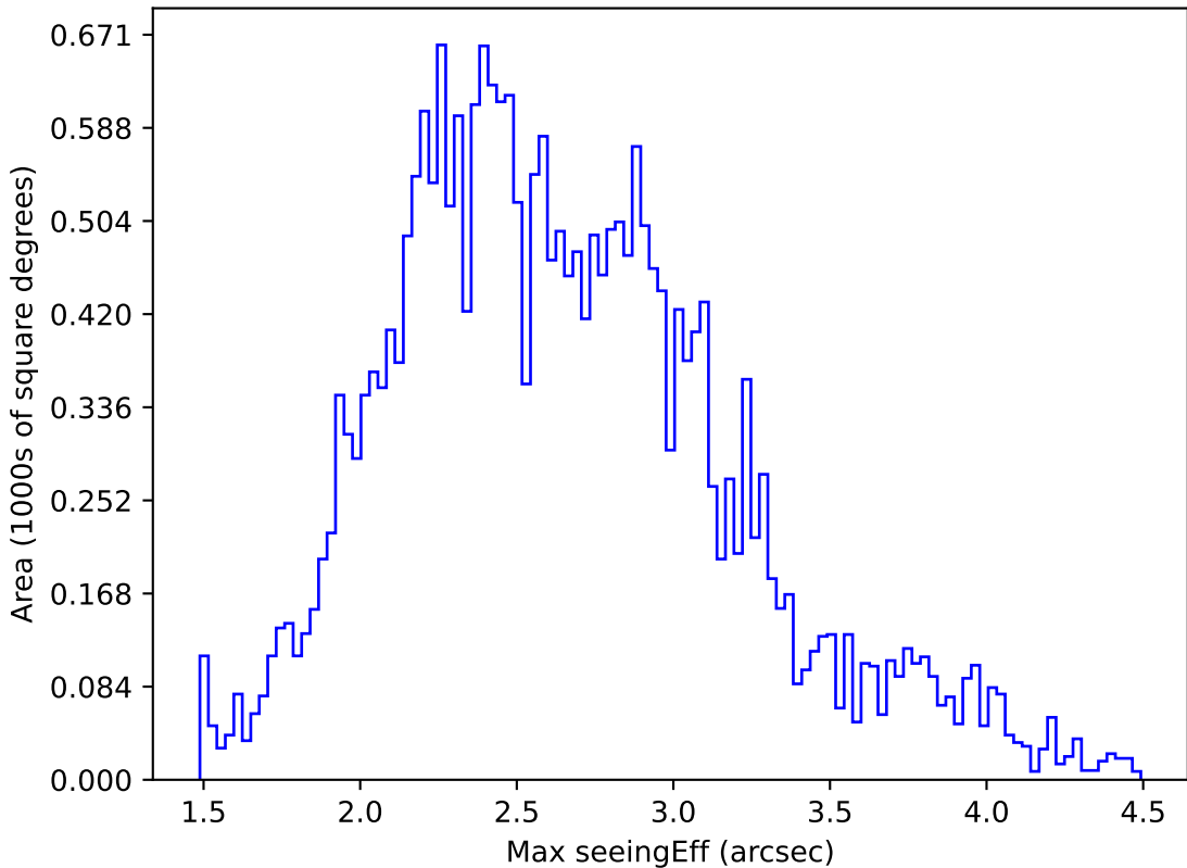
too_elab_heavy_r128_d2_gz_v3.4_10yrs All sky r band: Max seeingEff
