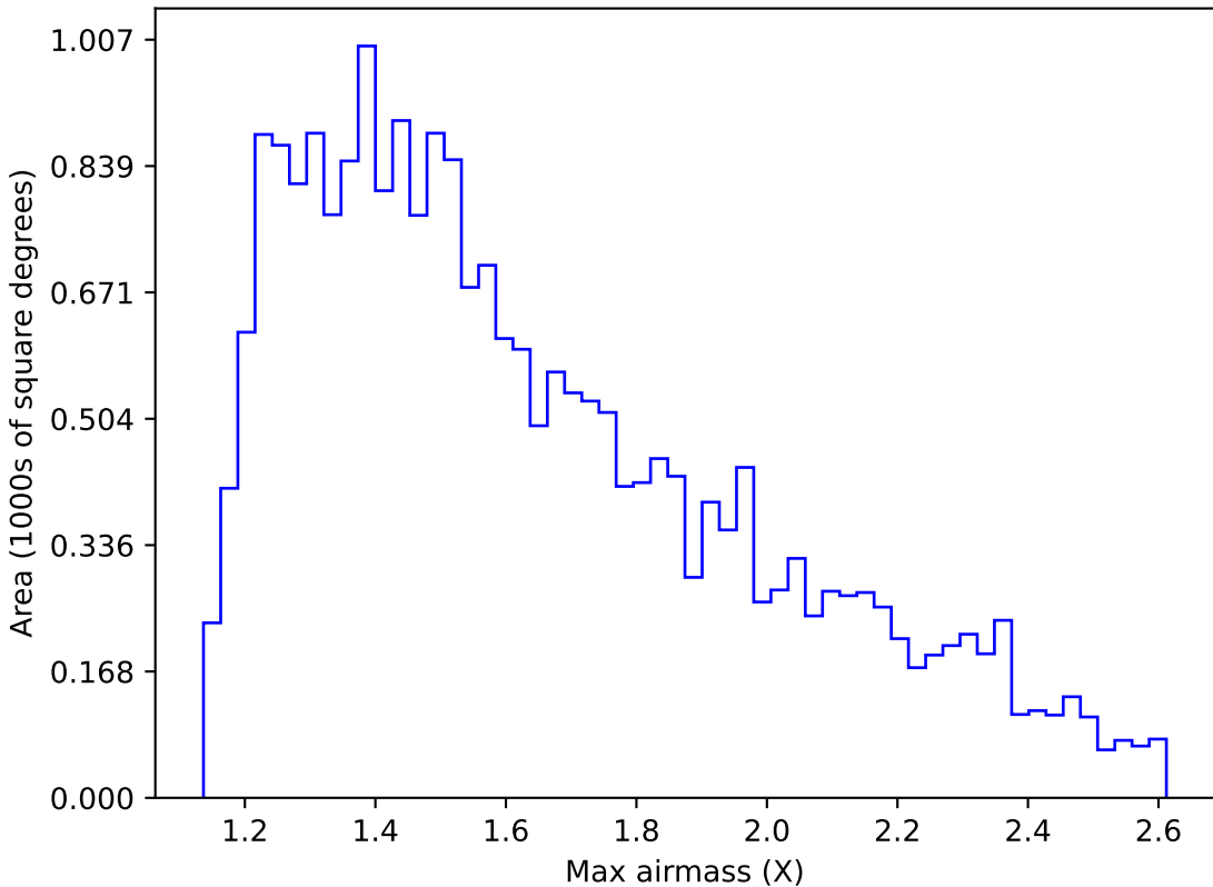
too_elab_heavy_r128_d2_gz_v3.4_10yrs Yr 1 y band: Max airmass
