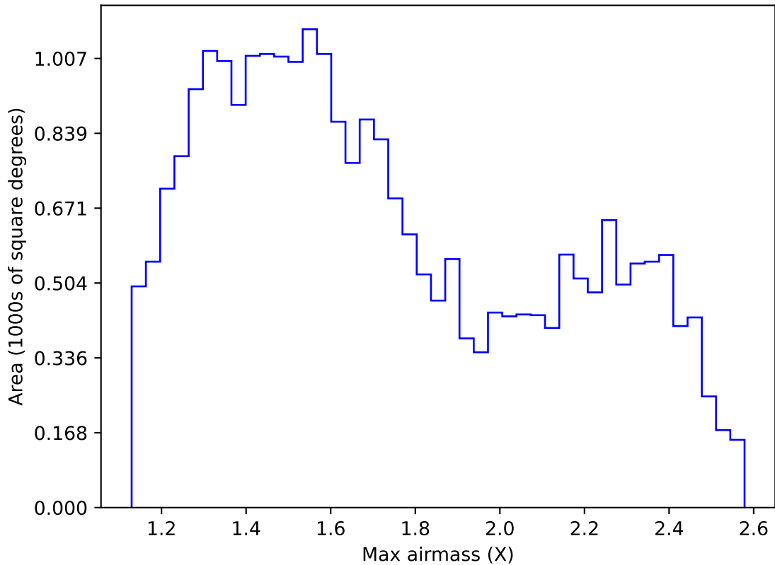
too_elab_heavy_r128_d2_gz_v3.4_10yrs Yr 1 r band: Max airmass
