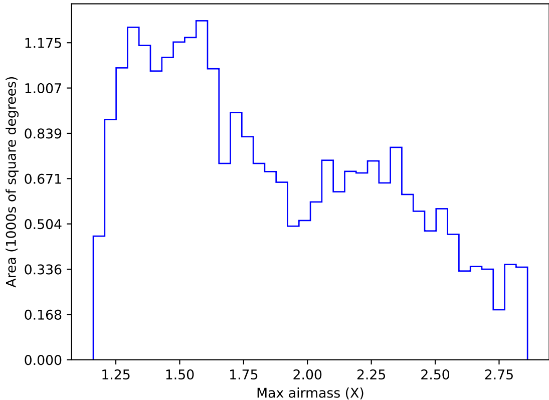
too_elab_heavy_r128_d2_gz_v3.4_10yrs Yr 1 i band: Max airmass
