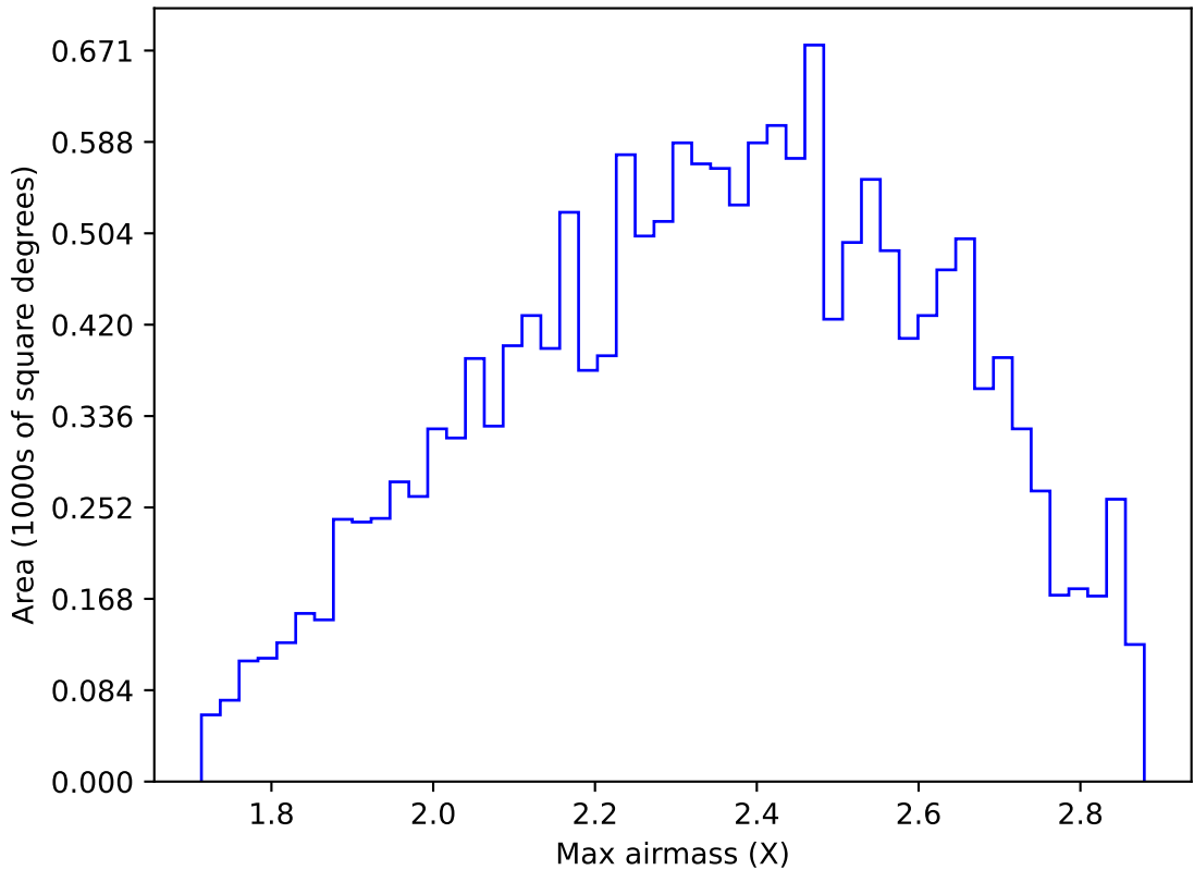
too_elab_heavy_r128_d2_gz_v3.4_10yrs WFD y band: Max airmass
