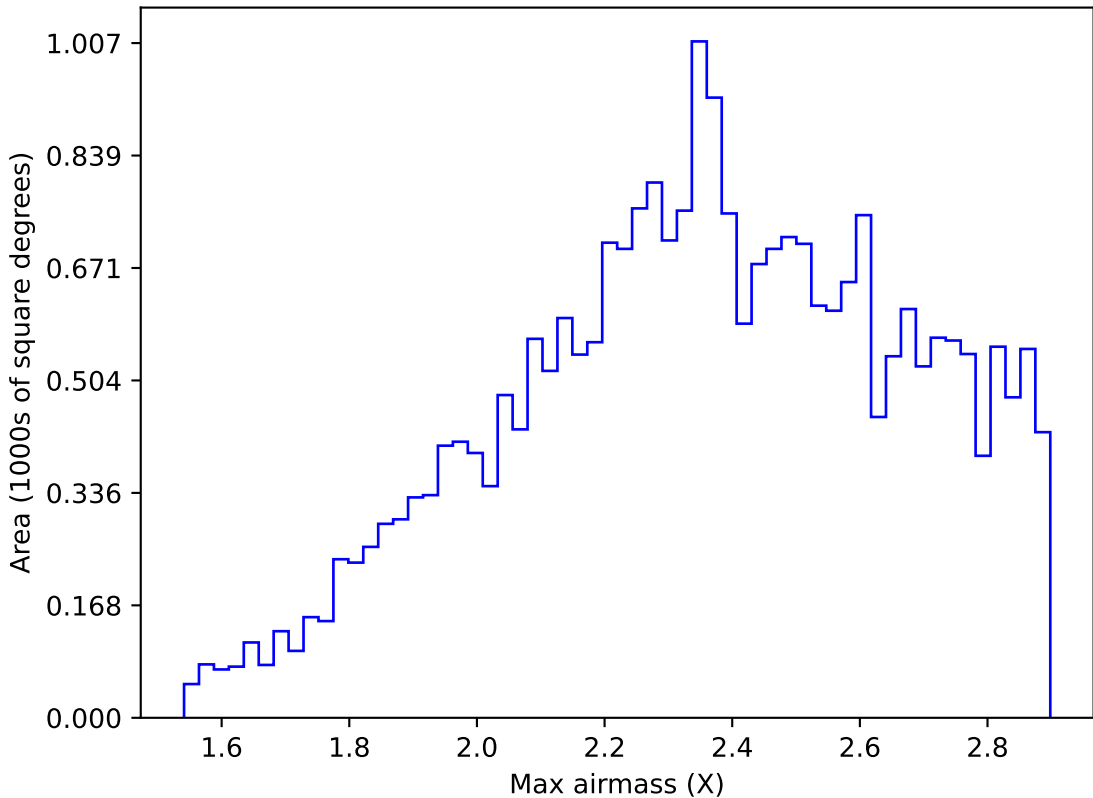
too_elab_heavy_r128_d2_gz_v3.4_10yrs All sky z band: Max airmass
