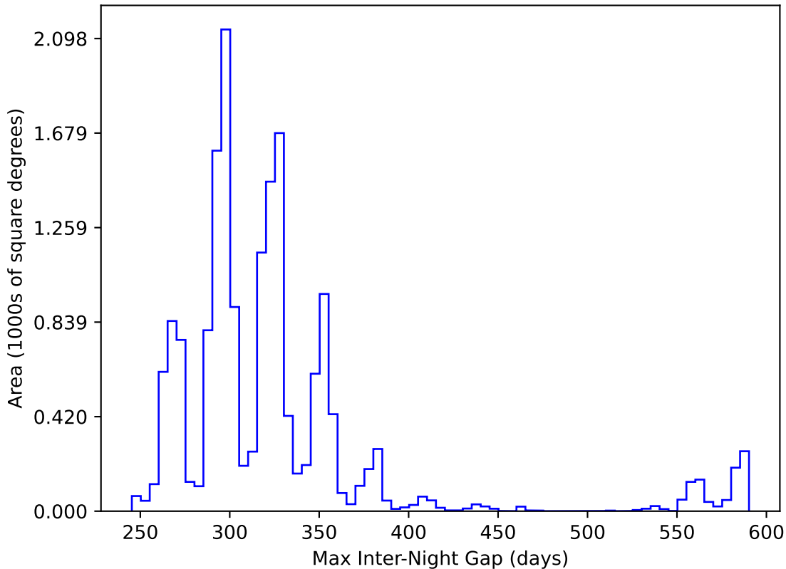
too_elab_heavy_r128_d2_gz_v3.4_10yrs WFD y band: Max Inter-Night Gap
