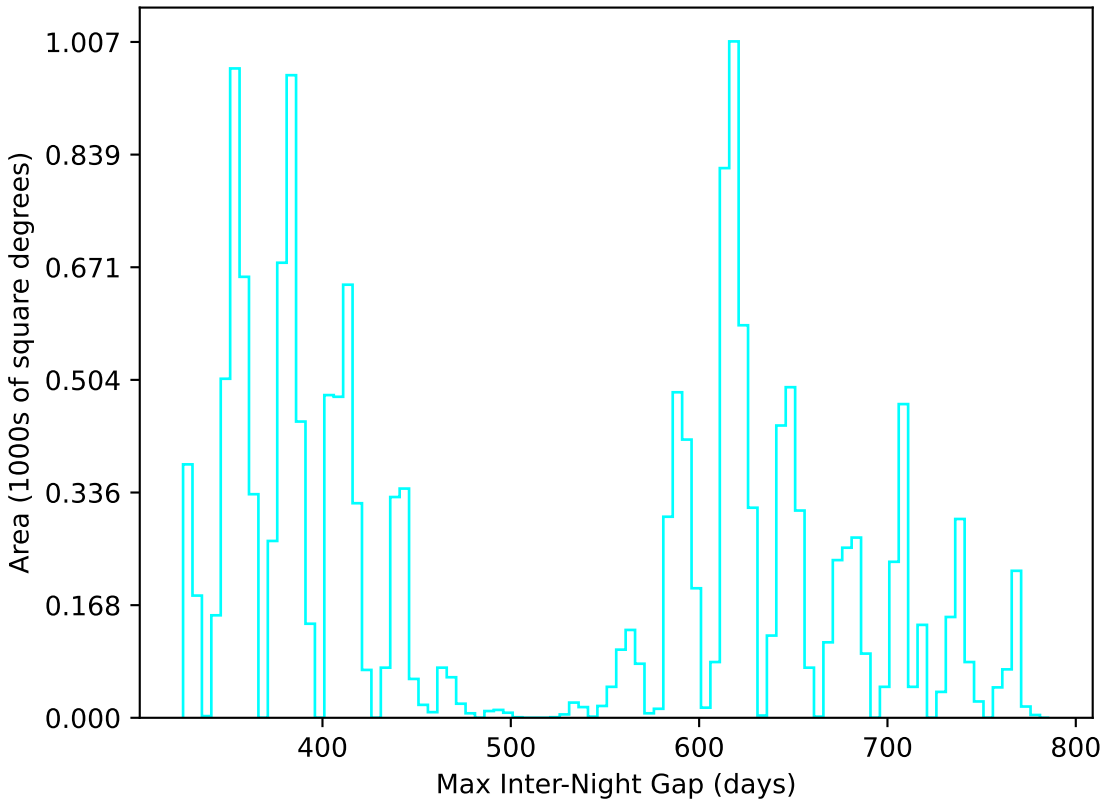
too_elab_heavy_r128_d2_gz_v3.4_10yrs WFD u band: Max Inter-Night Gap
