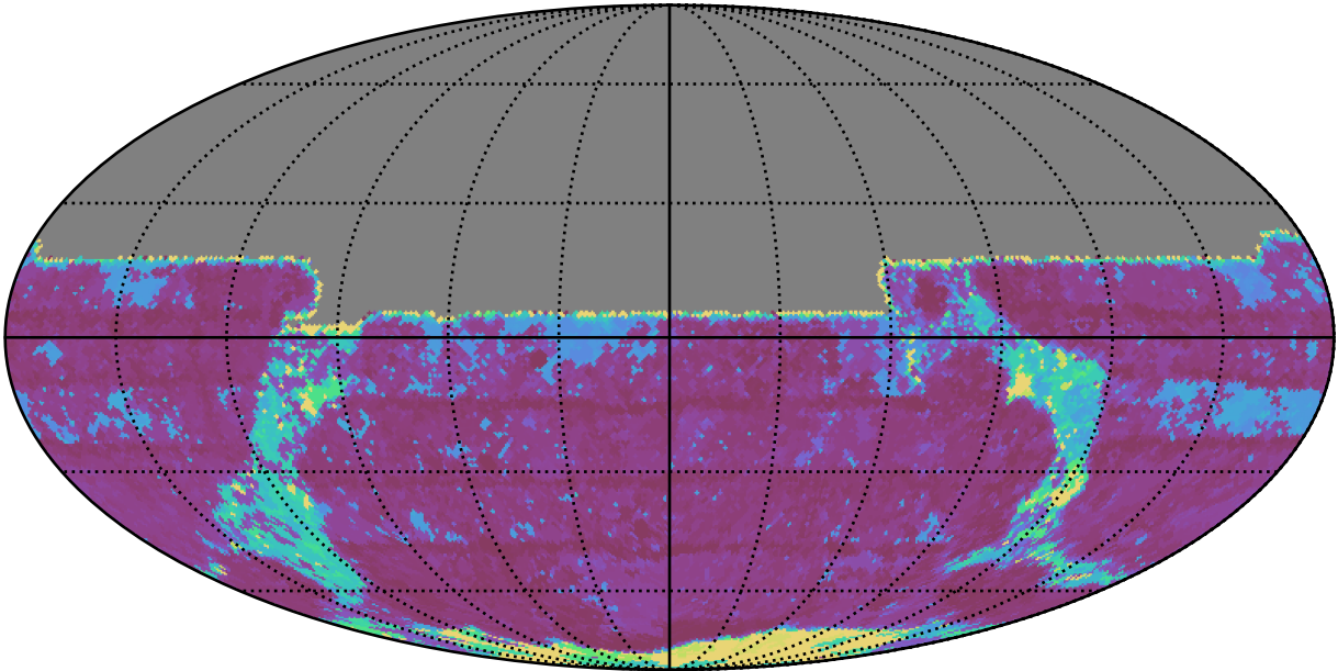
too_elab_heavy_r128_d2_gz_v3.4_10yrs All sky y band: Max Inter-Night Gap
