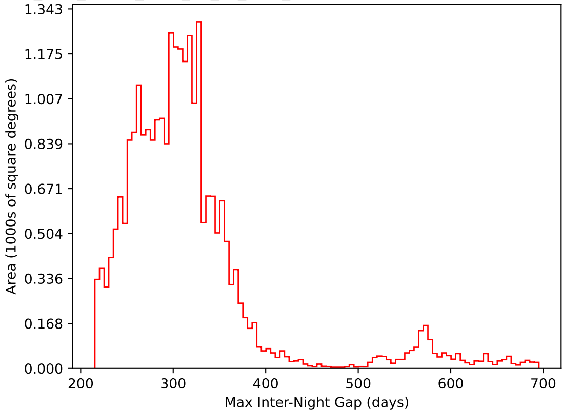
too_elab_heavy_r128_d2_gz_v3.4_10yrs All sky i band: Max Inter-Night Gap
