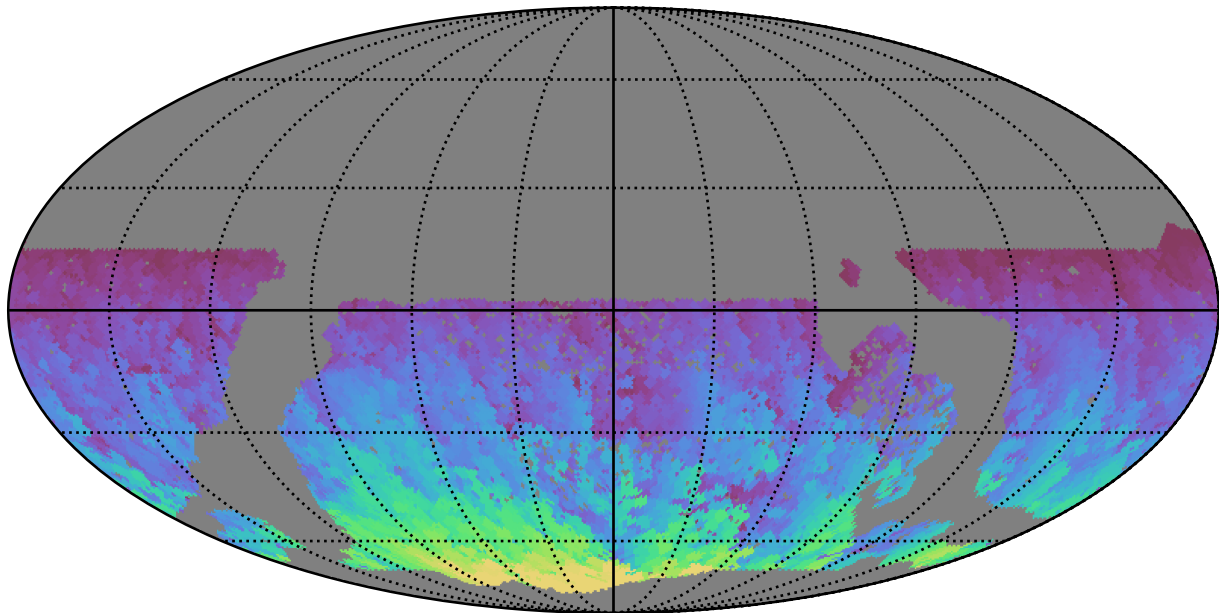
too_elab_heavy_r128_d2_gz_v3.4_10yrs WFD y band: Max HA
