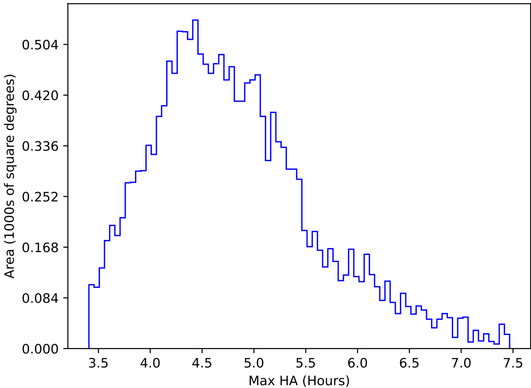
too_elab_heavy_r128_d2_gz_v3.4_10yrs WFD y band: Max HA
