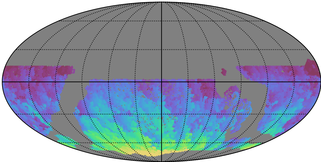
too_elab_heavy_r128_d2_gz_v3.4_10yrs WFD r band: Max HA
