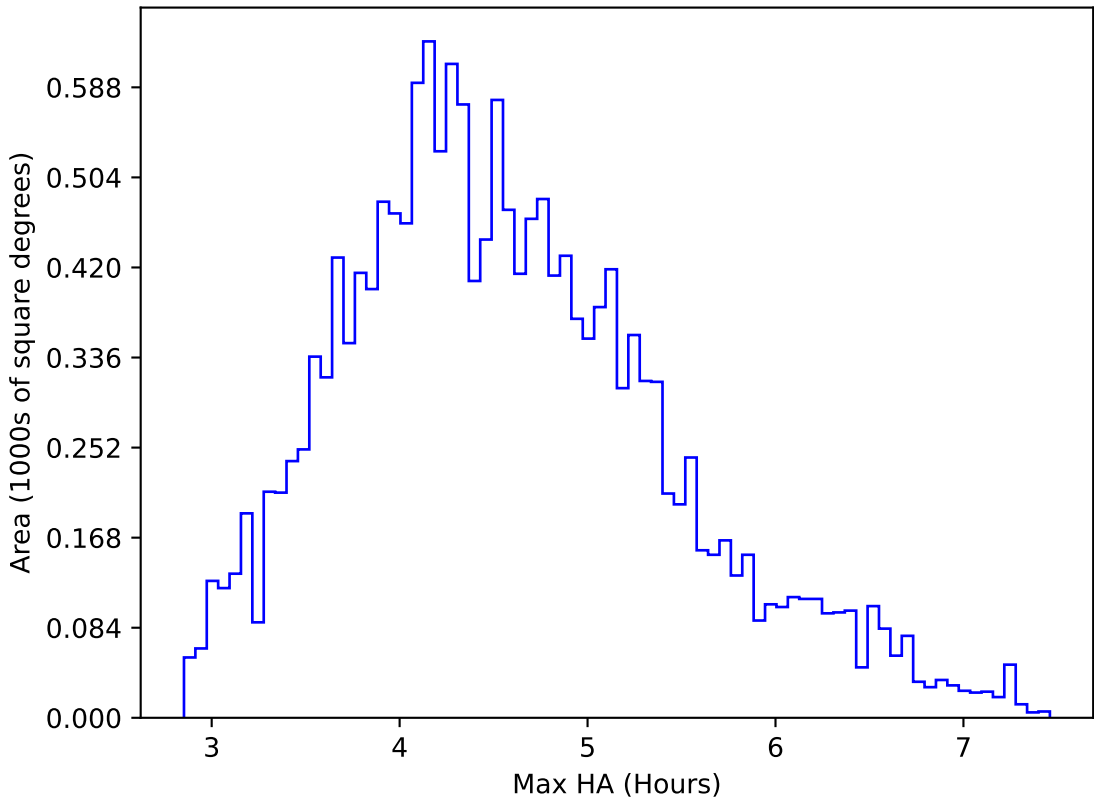
too_elab_heavy_r128_d2_gz_v3.4_10yrs WFD r band: Max HA
