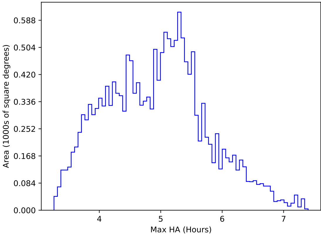
too_elab_heavy_r128_d2_gz_v3.4_10yrs WFD i band: Max HA
