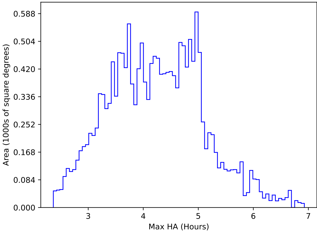
too_elab_heavy_r128_d2_gz_v3.4_10yrs WFD g band: Max HA
